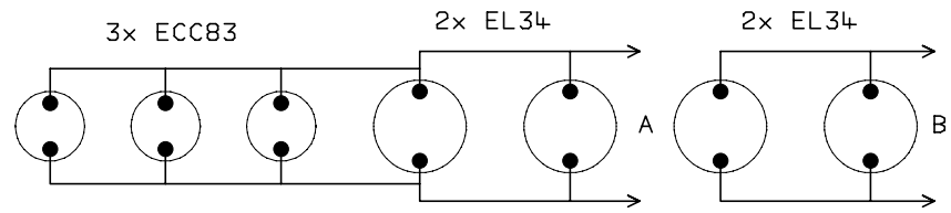
Valve Heater Wiring Arrangement
